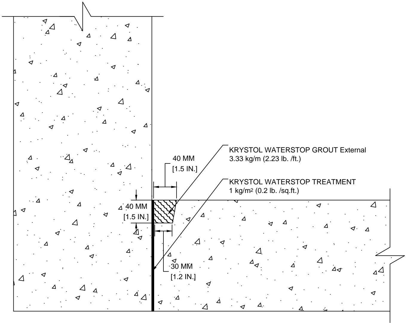
NEW CONSTRUCTION - WALL TO SLAB - SHOTCRETE (WALL INBOARD OF SLAB) REFER TO APPLICATION INSTRUCTION 4.21
